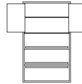
5-High Hinge Doors 2 Door Hinged 2 Receding 1 Drawer 1646mm H 800mm, 1000mm W
