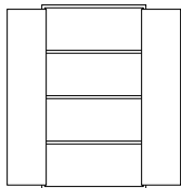
Hinged Doors 2-, 2.5-, 3-, 4-, 5-, 6-High 699mm, 857mm, 1016mm, 1330mm, 1646mm, 1964mm H 800mm, 1000mm W
