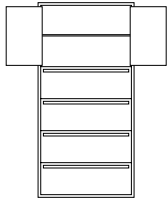
6-High Hinge Doors 2 Door Hinged 4 Drawers 1961mm H 800mm, 1000mm W
